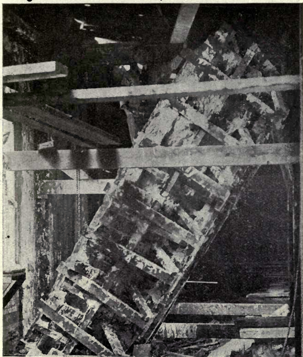
FIG. 45—TURNING CRADLE CONTAINING PLASTER MOLD FROM VERTICAL TO HORIZONTAL POSITION FOR FILLING WITH CONCRETE
